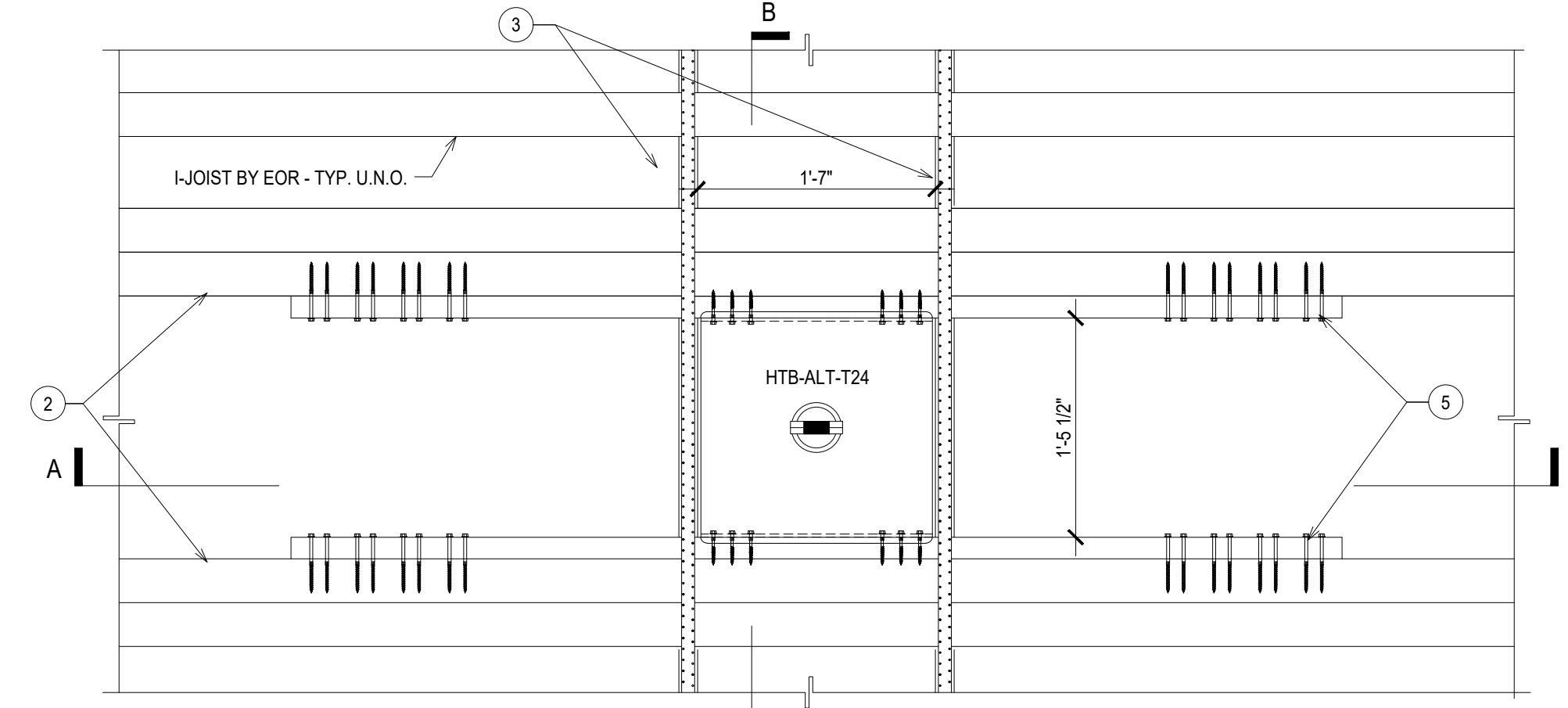
HTB-ALT LAYOUT DETAIL W/ WOOD TRUSS 2
