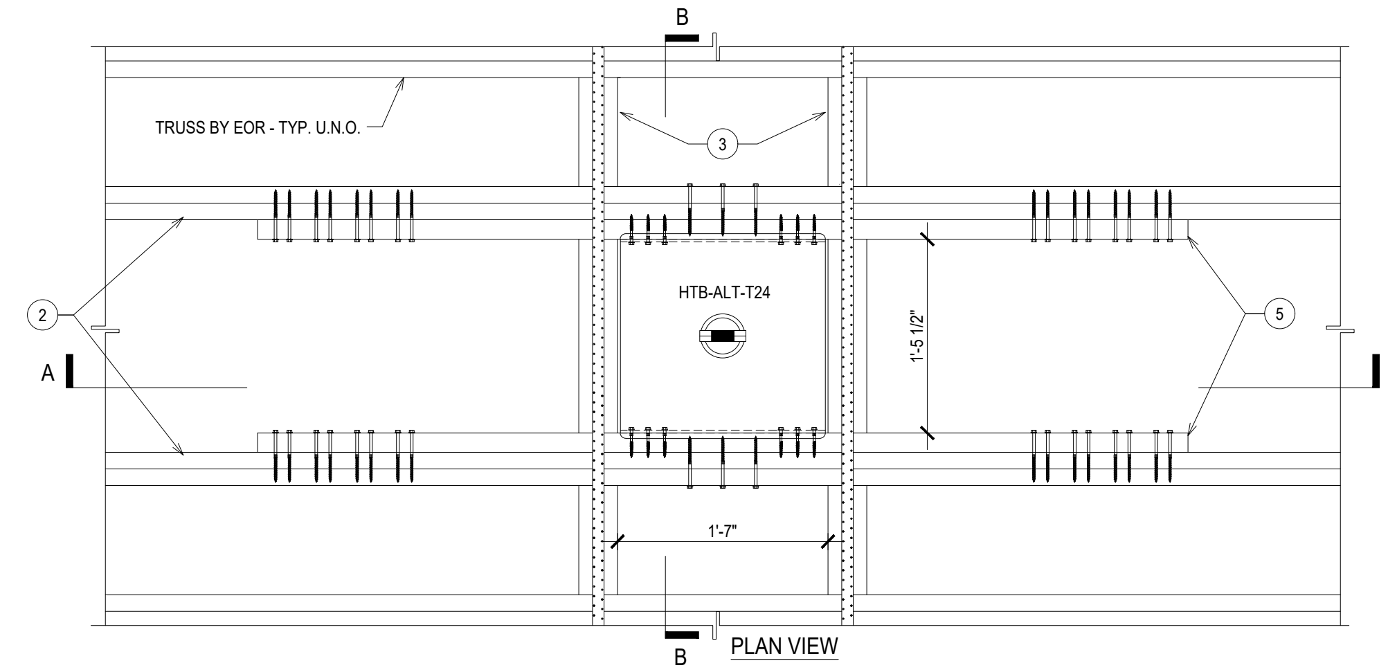
HTB-ALT LAYOUT DETAIL W/ WOOD TRUSS 2
