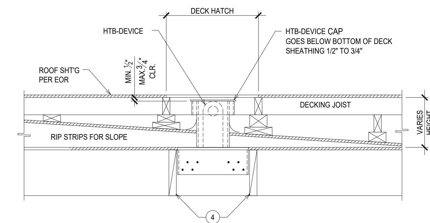
HTB-ALT-CM LAYOUT BELOW ROOF DECK ABV RIP STOPS 3
