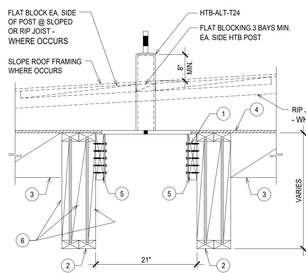
SECTION B-B
